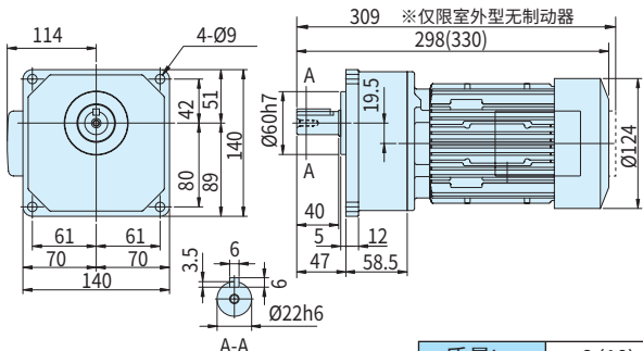
图C11 ZNFM05-1220-3~30 (ZNFM05-1220-B-3~30)
