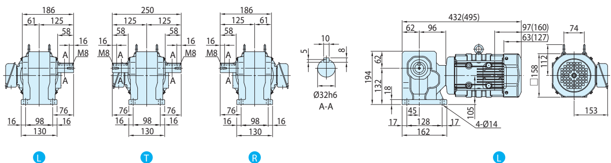
图E436 RNHM1-50 \frac{1}{2} -EP-80~120 (RNHM1-50 \frac{1}{2} -EP-B-80~120)
