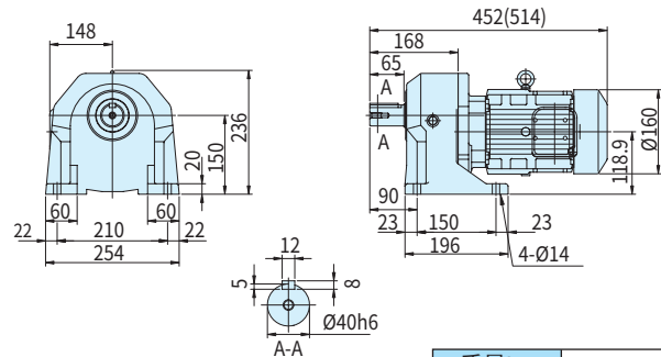
图C32 ZNHM2-1401-30~100 (ZNHM2-1401-B-30~100)
