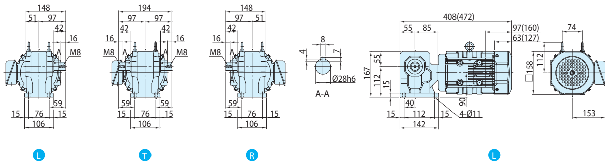
图E435 RNHM1-43 \frac{1}{2} -EP-40~60 (RNHM1-43 \frac{1}{2} -EP-B-40~60)
