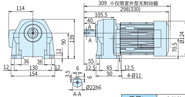
图C12 ZNHM05-1220-3~30 (ZNHM05-1220-B-3~30)
