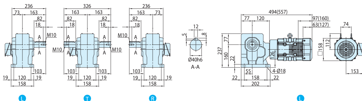
图E438 RNHM1H-470 \frac{1}{2} -EP-5~30 (RNHM1H-470 \frac{1}{2} -EP-B-5~30)
