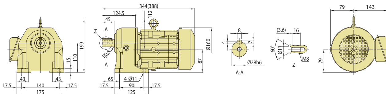
图 C45 ZNHM05-1280-EP-3~30 (ZNHM05-1280-EP-B-3~30)
