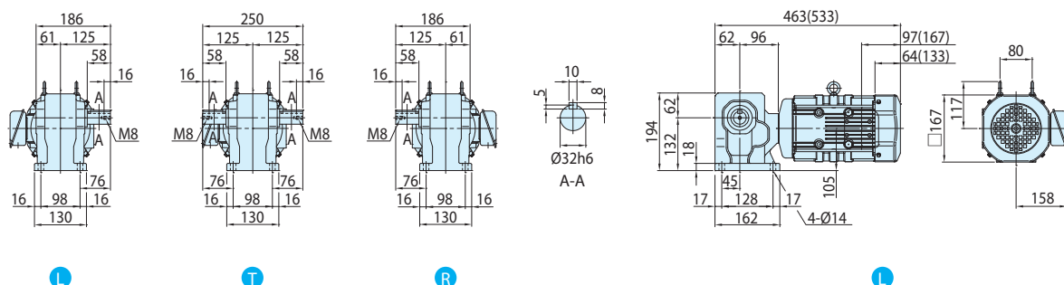
图E439 RNHM1H-53 \frac{1}{2} -EP-40~80 (RNHM1H-53 \frac{1}{2} -EP-B-40~80)
